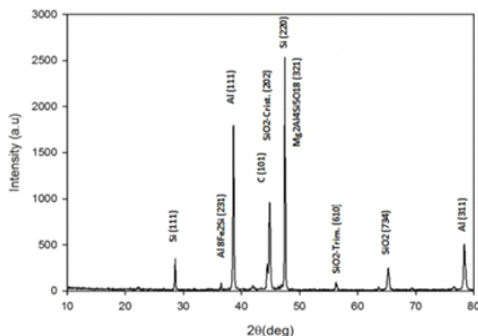
Fig. 5. XRD of Al-alloy-RHA composite.
