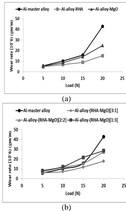
Fig. 8. Wear rate (a) Al-master alloy, Al- alloy-RHA and Al-alloy-MgO composites, and (b) Al-master alloy, Al- alloy-(RHA-MgO) hybrid composites.
