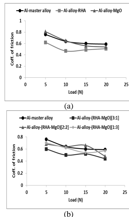
Fig. 9. COF (a) Al-master alloy, Al- alloy-RHA and Al- alloy-MgO composites, and (b) Al-master alloy, Al- alloy-(RHA-MgO) hybrid composites.
