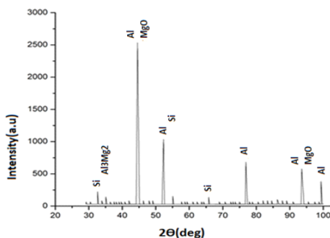
Fig. 6. XRD of Al-alloy-MgO.
